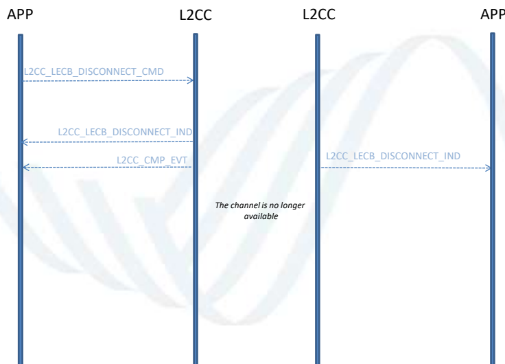
Figure 4-3: Disconnection of a LE Credit Based Connection.
