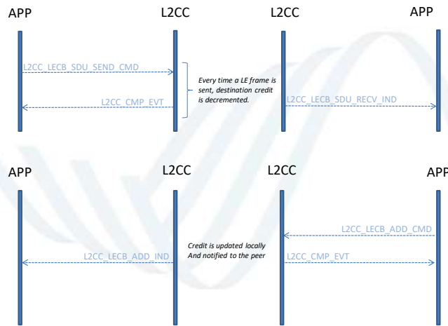
Figure 4-2: SDU transmission and reception over LECB Link and flow control
