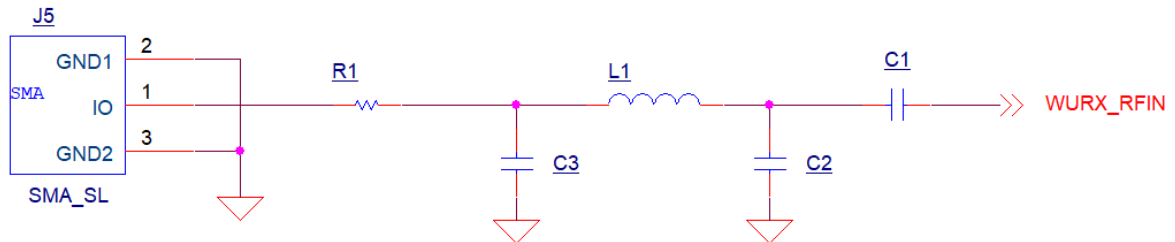
Figure 7 - Wakeup Radio Matching Circuit
