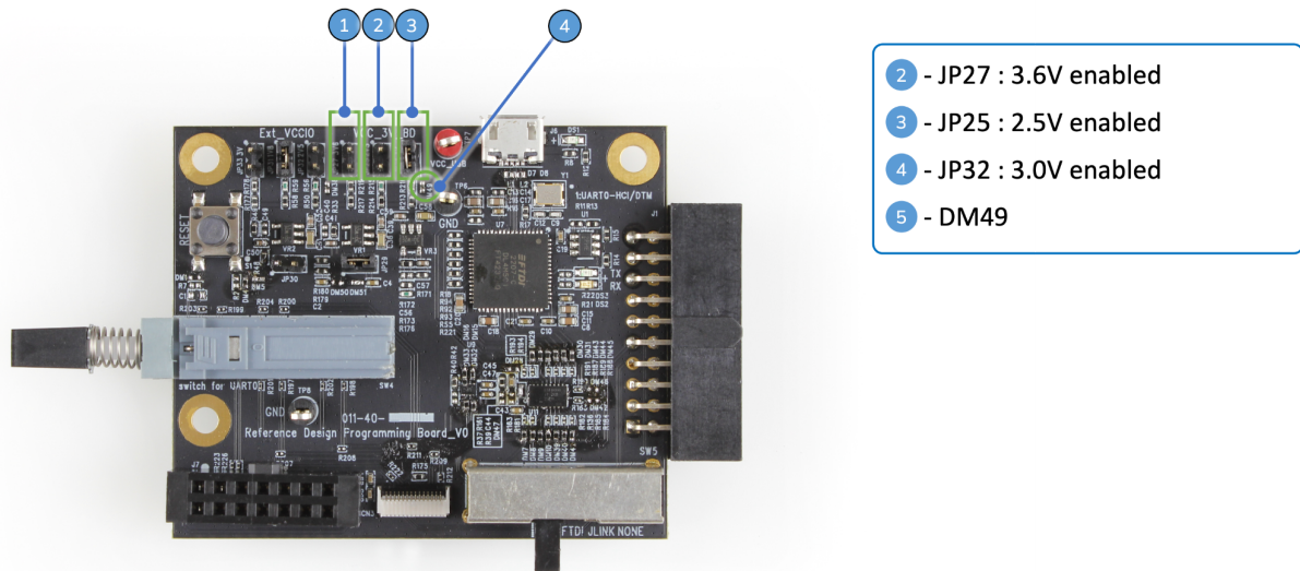
Figure 8 - Detail for VCC Source Section
