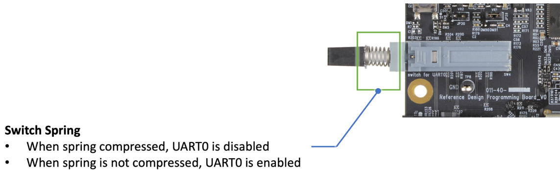
Figure 9 - Push Switch for UART0 Control
