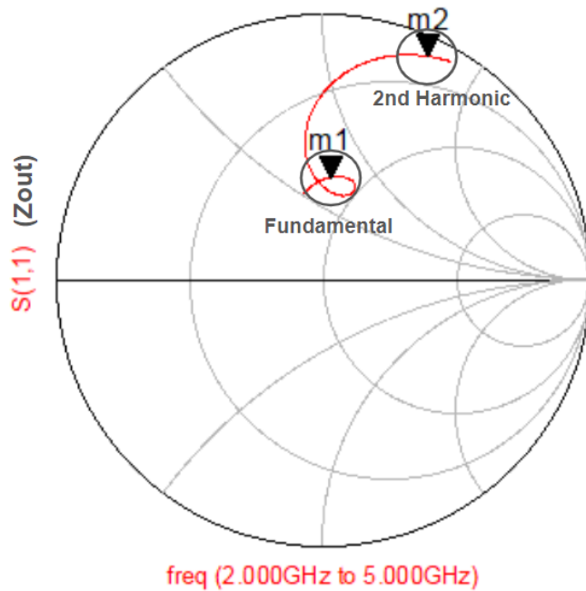
Figure 6-3 - Simulated RFIO Match S11 Looking Out from the SoC
