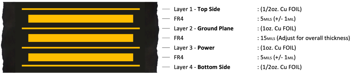
Figure 6-5 - 4-Layer Stack-up for Thinner PCB
