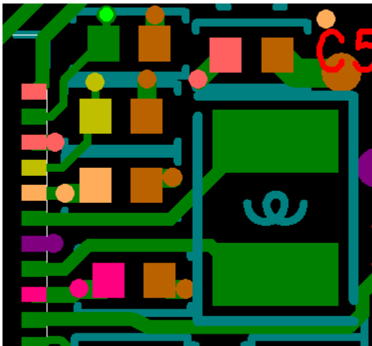
Figure 6-7 - Switcher Inductor Layout Recommendation for ATM3430 or ATM3430e PCB
