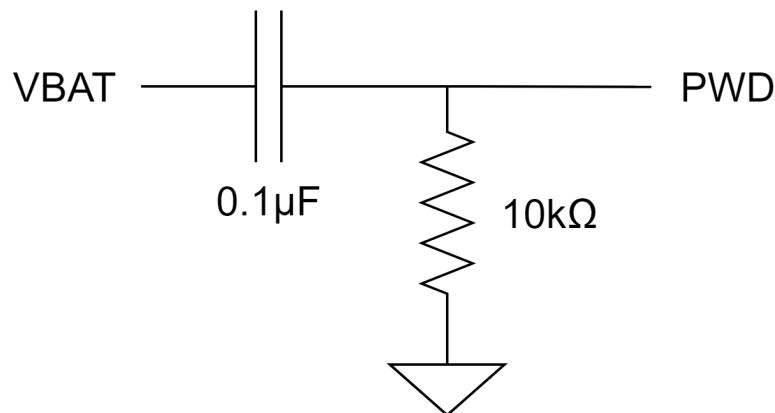
Figure 4-1 - Circuit to Generate PWD Pulse
