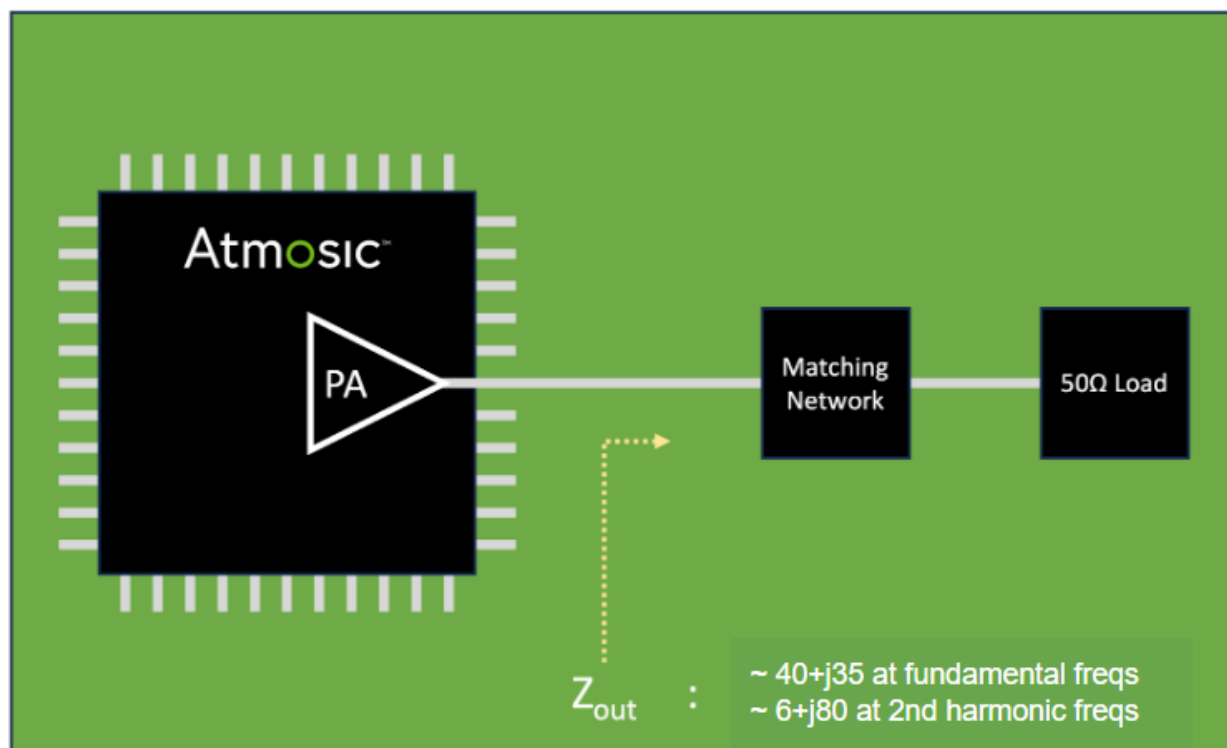
Figure 6-2 - RFIO Match Circuit Block Diagram
