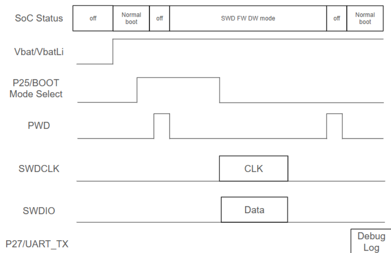
Figure 7-1 SWD signal timing sequence
