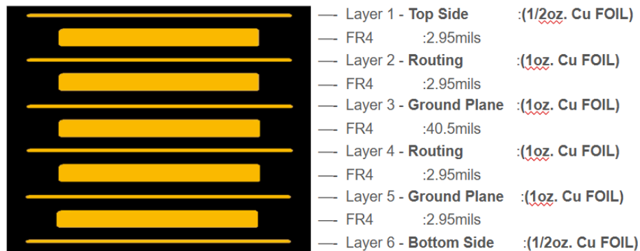
Figure 6-6 - 6-Layer Stack-up for ATM3405 BGA EVB
