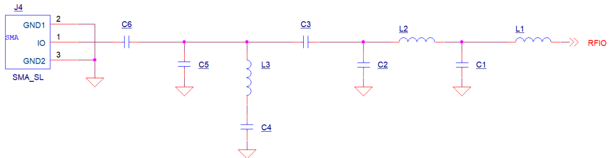
Figure 6-1 - RFIO Matching Circuit
