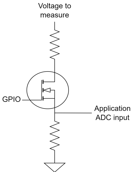
Figure 4-2 - Voltage Divider with a Transistor for Application ADC
