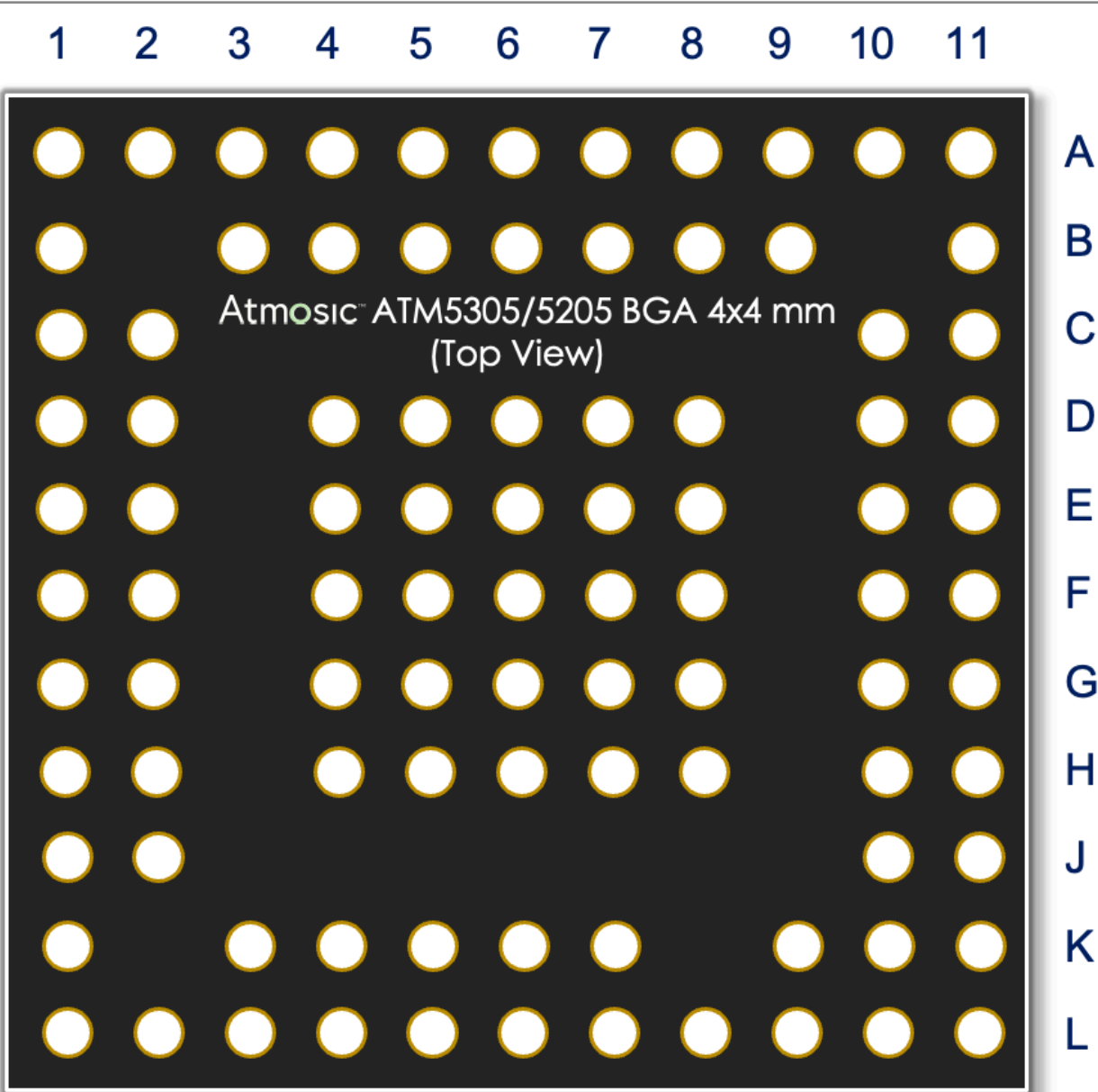
Figure 3.1-2 ATM5305 and ATM5205 4x4 mm, 93-ball BGA Pinout (Bottom View)
